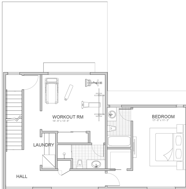
2ND FLOOR PLAN 1/4"=1'-0"
