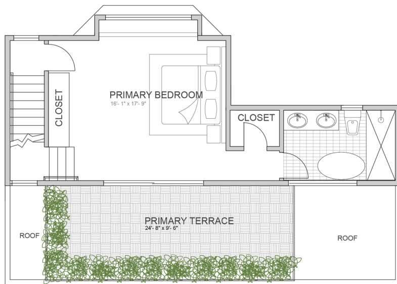
3R FLOOR PLAN 1/4"=1'-0"
