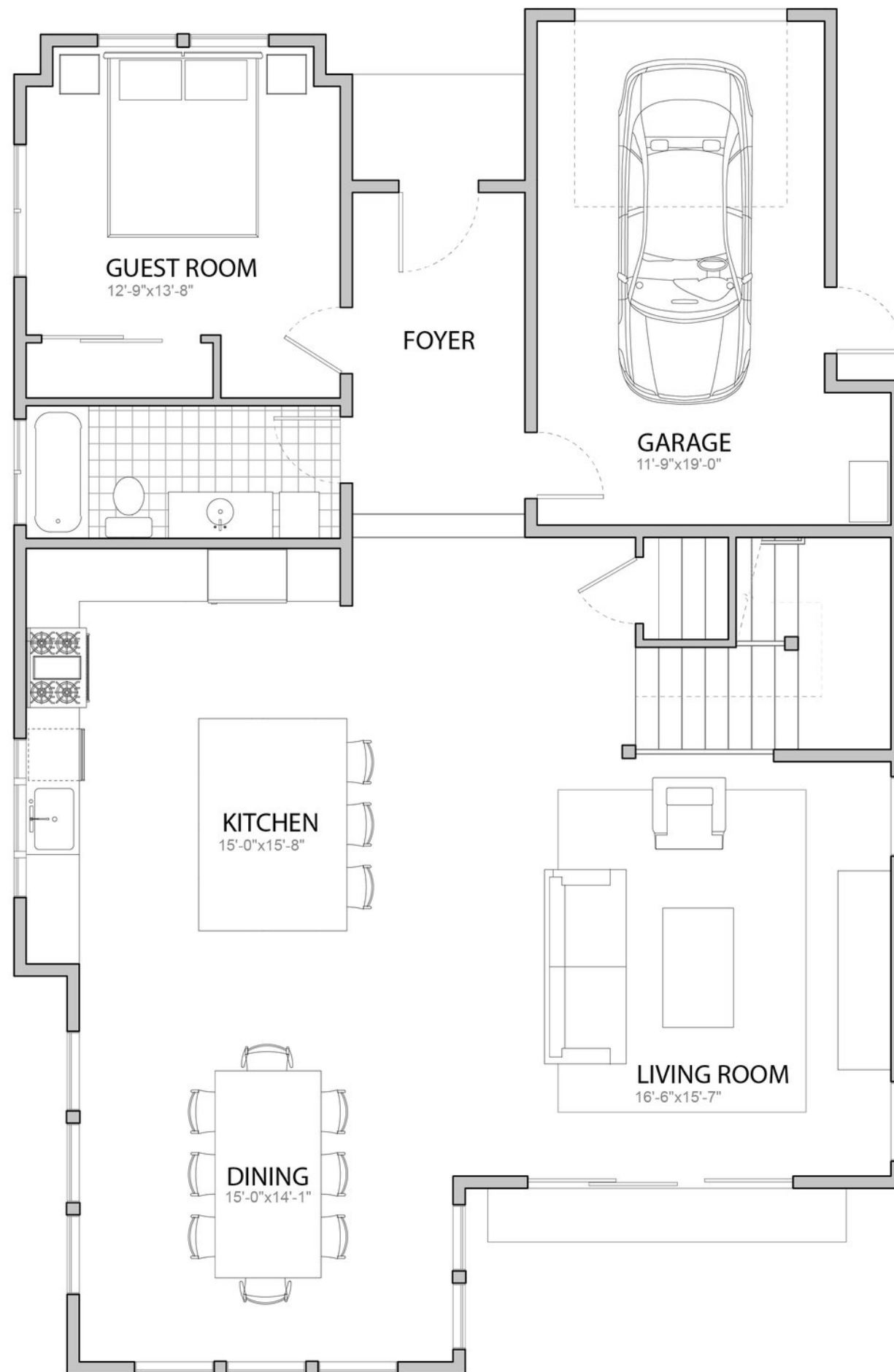
345 - 1st FLOOR PLAN
