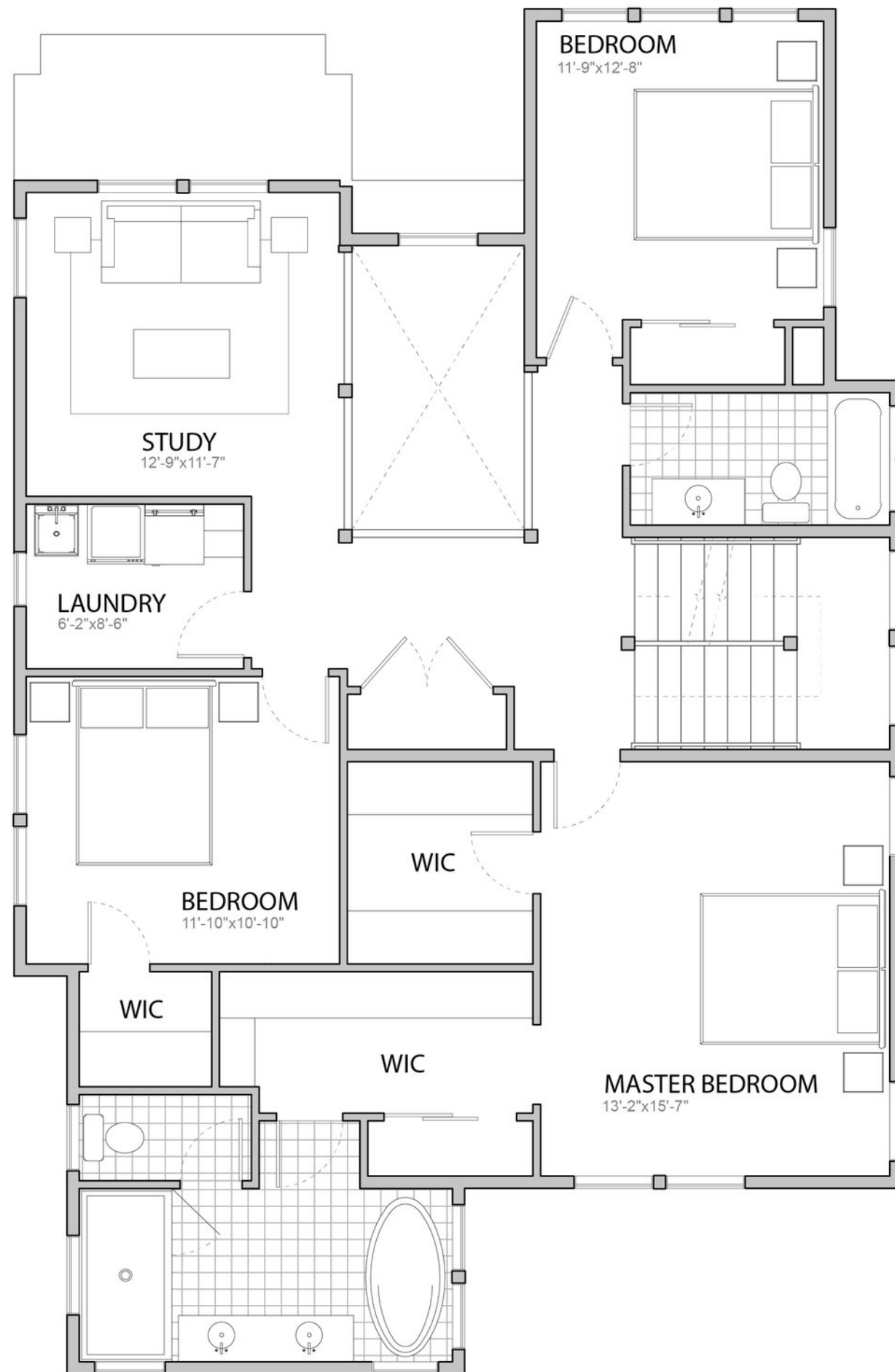
345 - 2nd FLOOR PLAN
